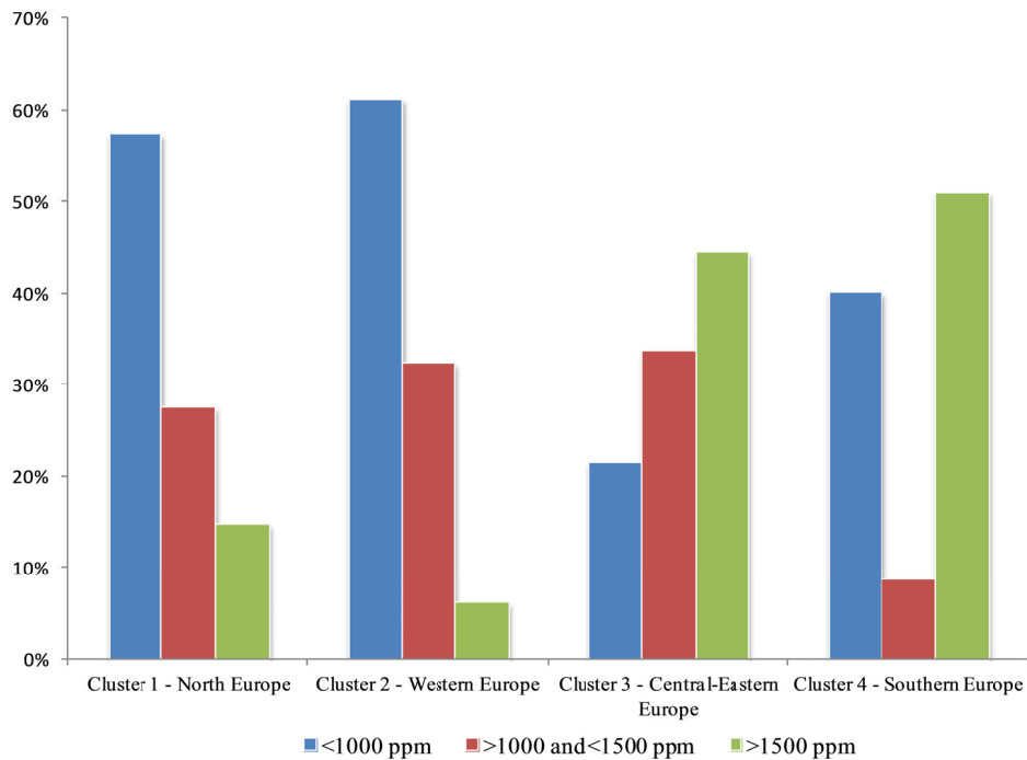
Figure 33. Distribution of CO 2 concentrations by SINPHONIE cluster
