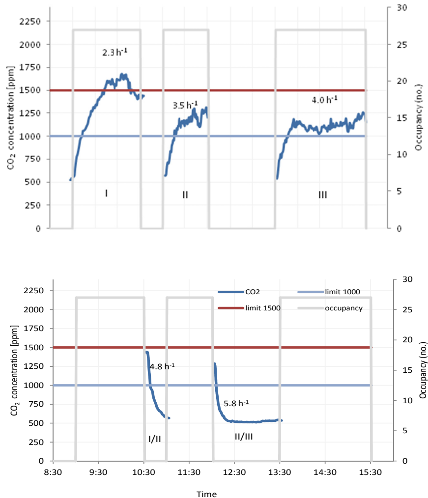
Figure 47. Evolution of CO 2 concentrations in a classroom during the second day of the measurement campaign
